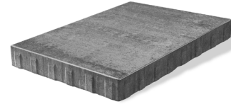
SLAB 22 7/16 x 37 3/8 x 2 3/8" 570 x 950 x 60mm See Slabs section page 84 for more details.
